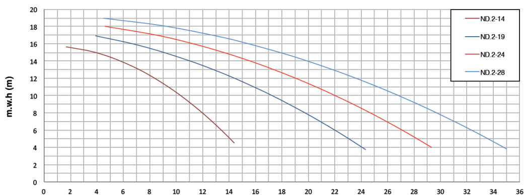
Characteristics curve
